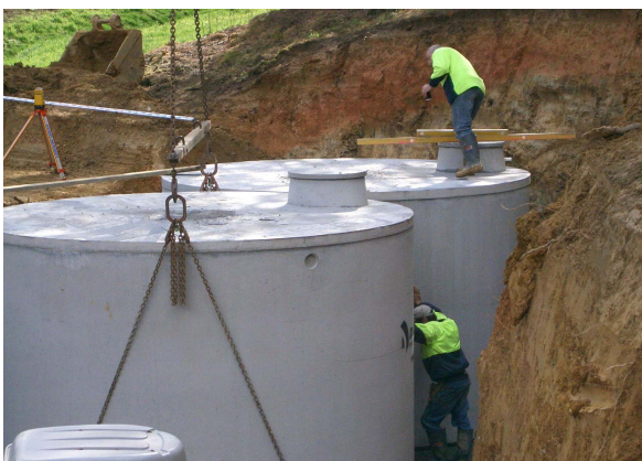
25,000L Underground Attenuation Tank
