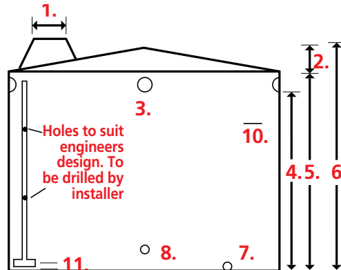
Standard 25,000L Tank Unequally Buried
